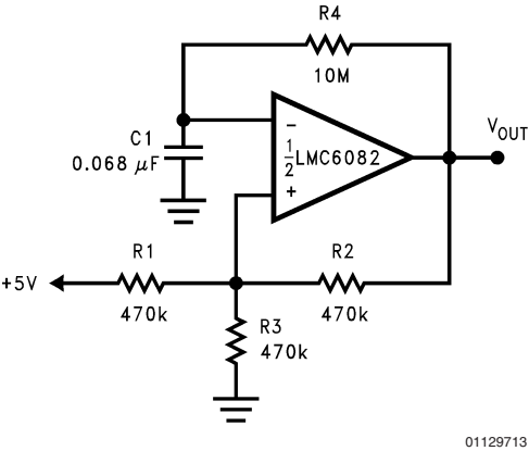
FIGURE 9. 1 Hz Square Wave Oscillator
